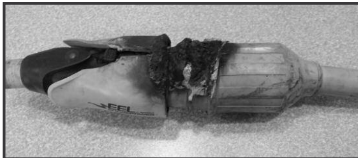
Potential fire hazard: a damaged 50A power cord without a waterproof collar.
